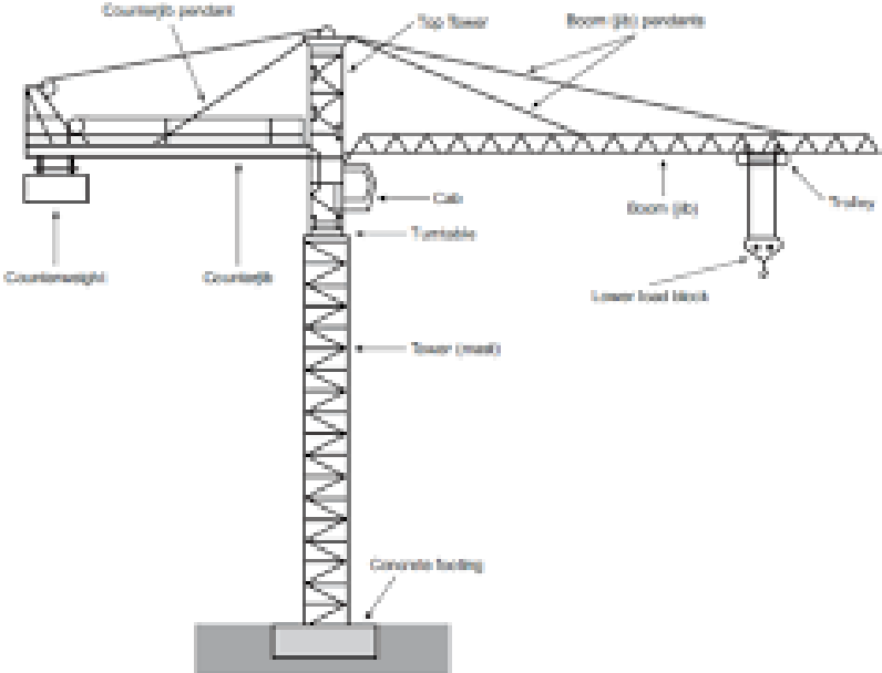
Tower Crane - Hammerhead
